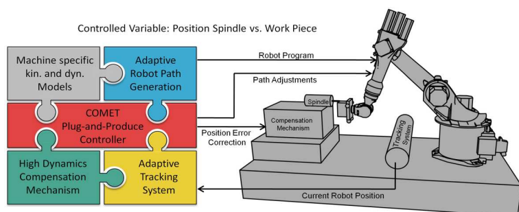
2. The complete COMET platform for high accuracy machining with robots
