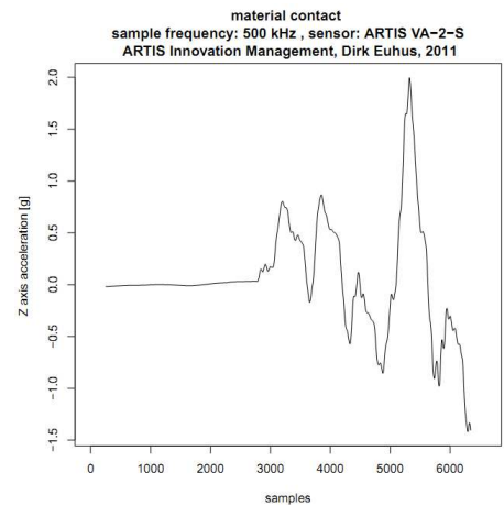
3. Z acc. before and after metal contact
